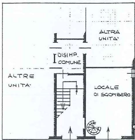
PIANO TERRA H = 2,40
